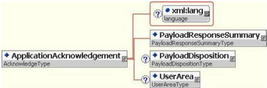
Figure 1 : Le type AcknowledgeType
