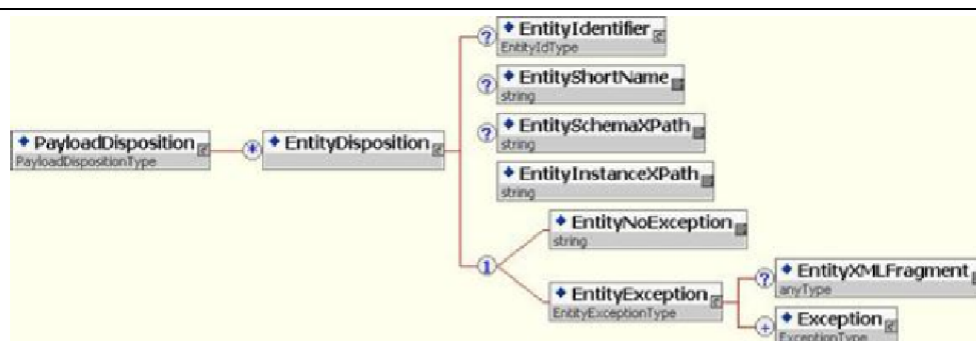
Figure 3 : Le type PayloadDispositionType
